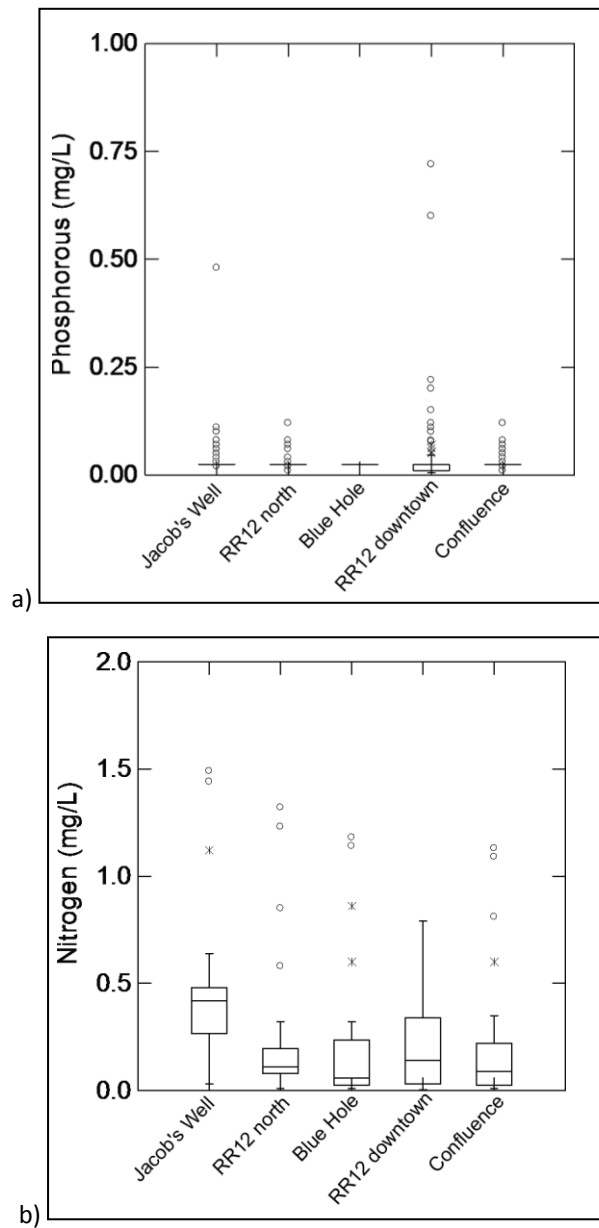
Figure 6.2 (a,b). Phosphorus and nitrogen data.
