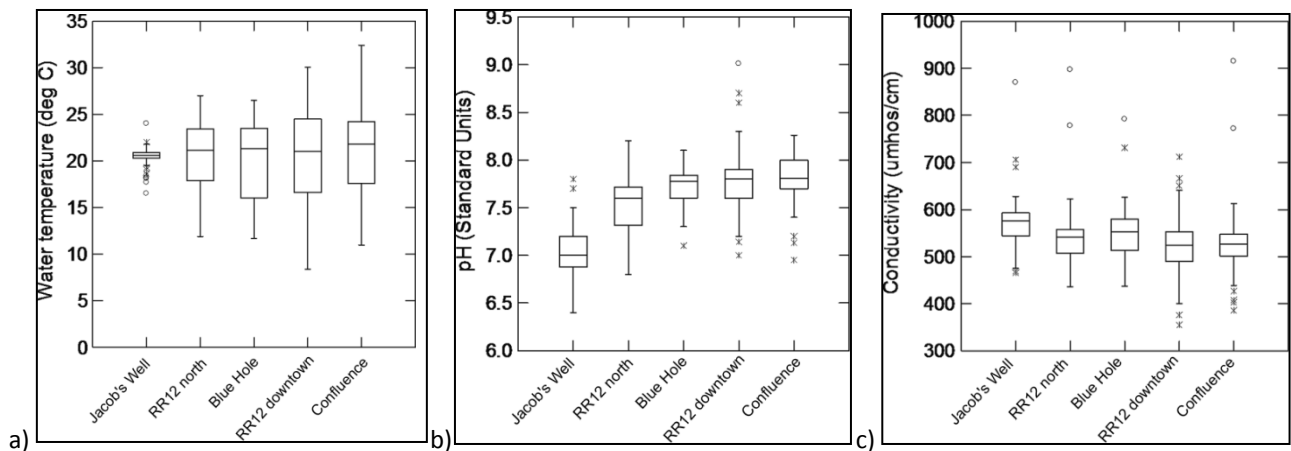
Figure 6.1 (a,b,c). Water chemistry-related parameters.
