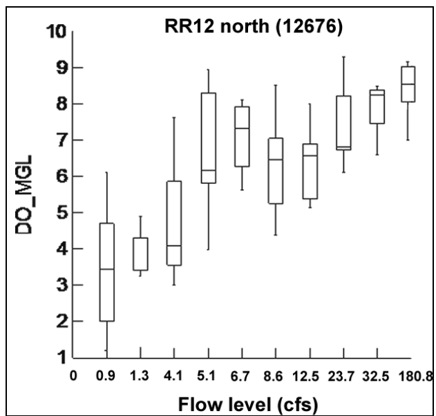
Figure 6.15. DO concentrations at RR12 north by flow level.
