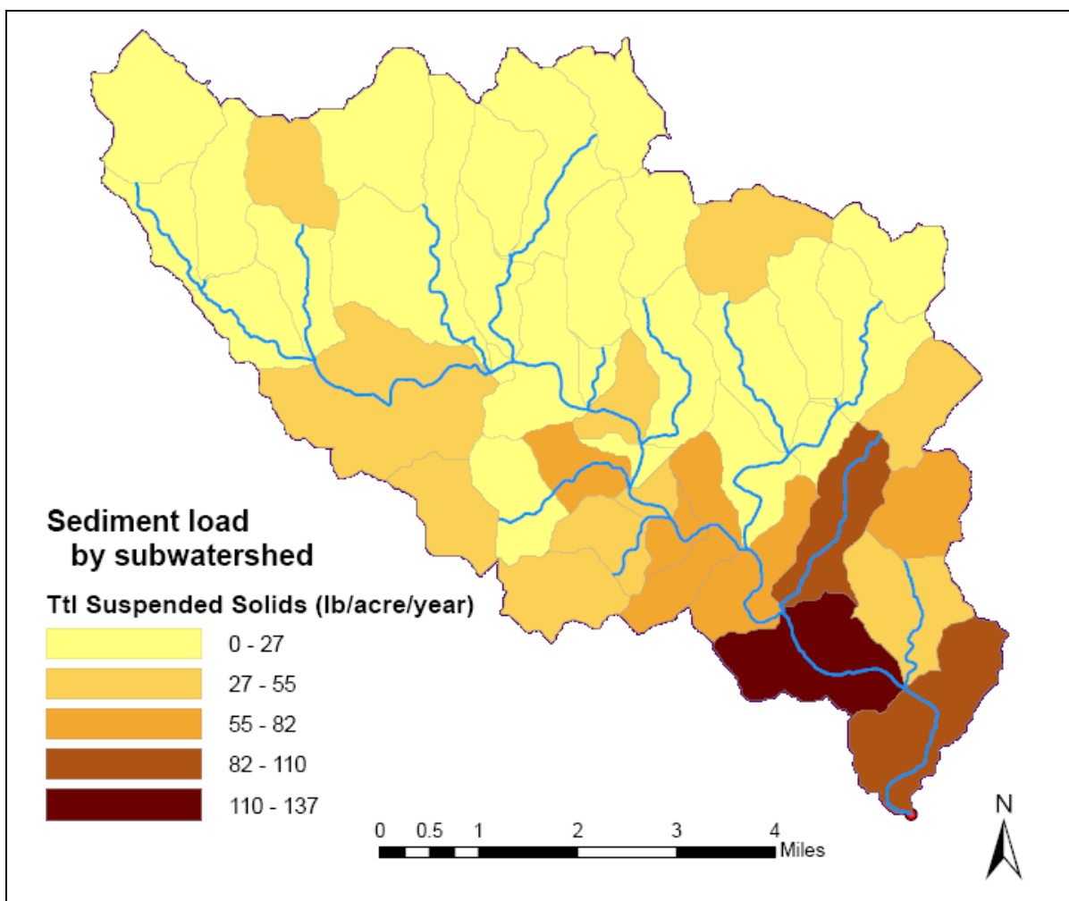
Figure 5.7. Total suspended solids, estimated load by subwatershed.
