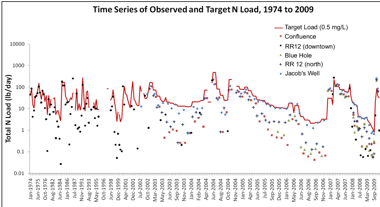
Figure 6.5. Time series of observed and target nitrogen load for five sites along Cypress Creek.
