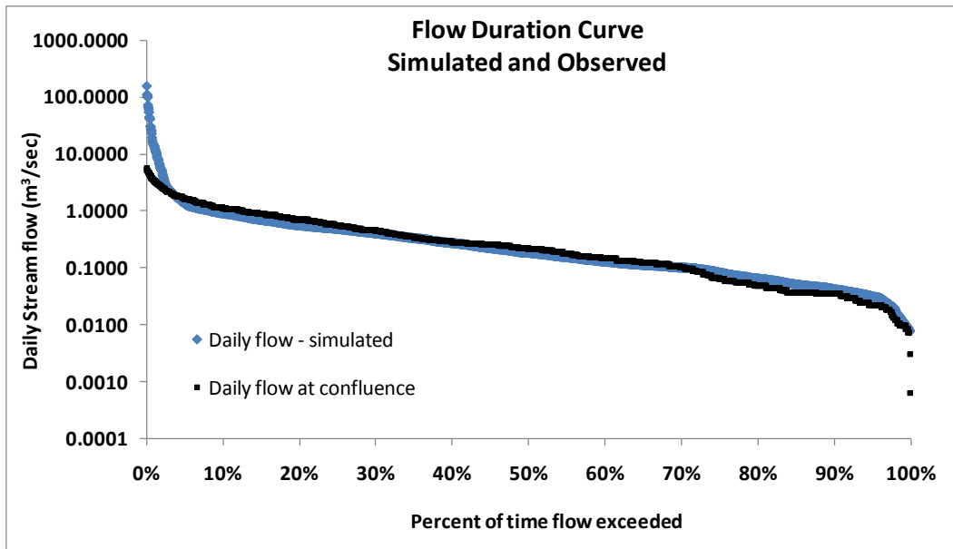
Figure B.1. Simulated and Observed Flow Duration Curves for the Cypress Creek watershed. Daily flows ( m^3/sec ) were simulated using the SWAT2000 hydrologic model.
