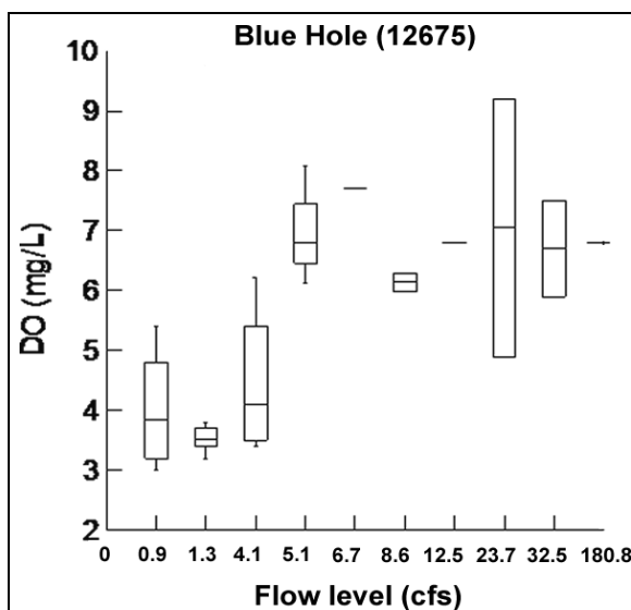
Figure 6.16. DO concentrations at Blue Hole by flow level.
