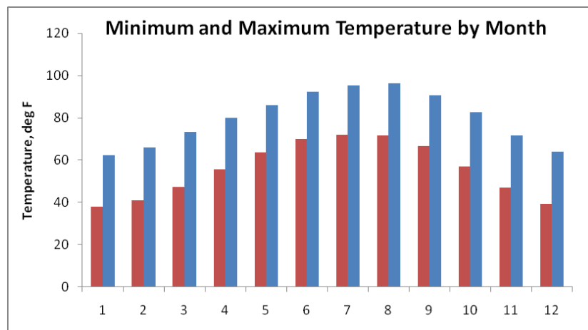
Figure 2.3. Monthly temperature ranges in Cypress Creek watershed.
