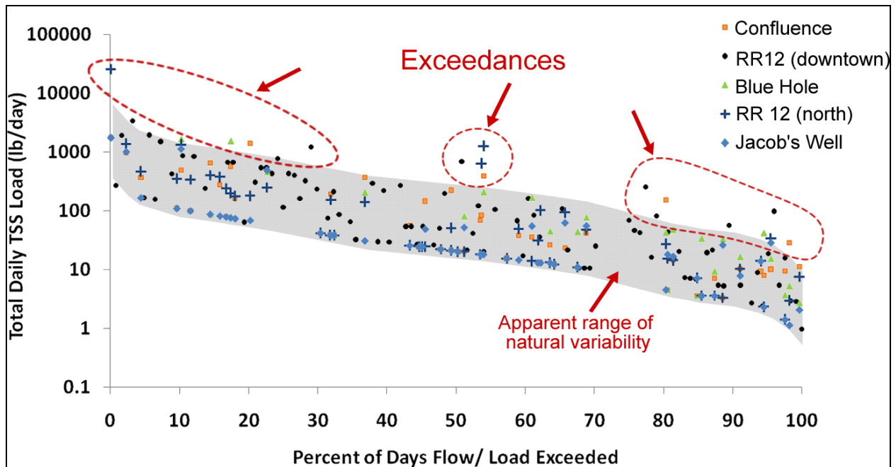
Figure 6.8. Load duration curve of total suspended solids (sediment) at five sites along Cypress Creek.
