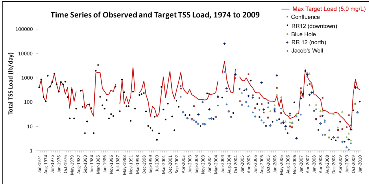
Figure 6.10. Time series of observed and target maximum sediment load for five sites along Cypress Creek.
