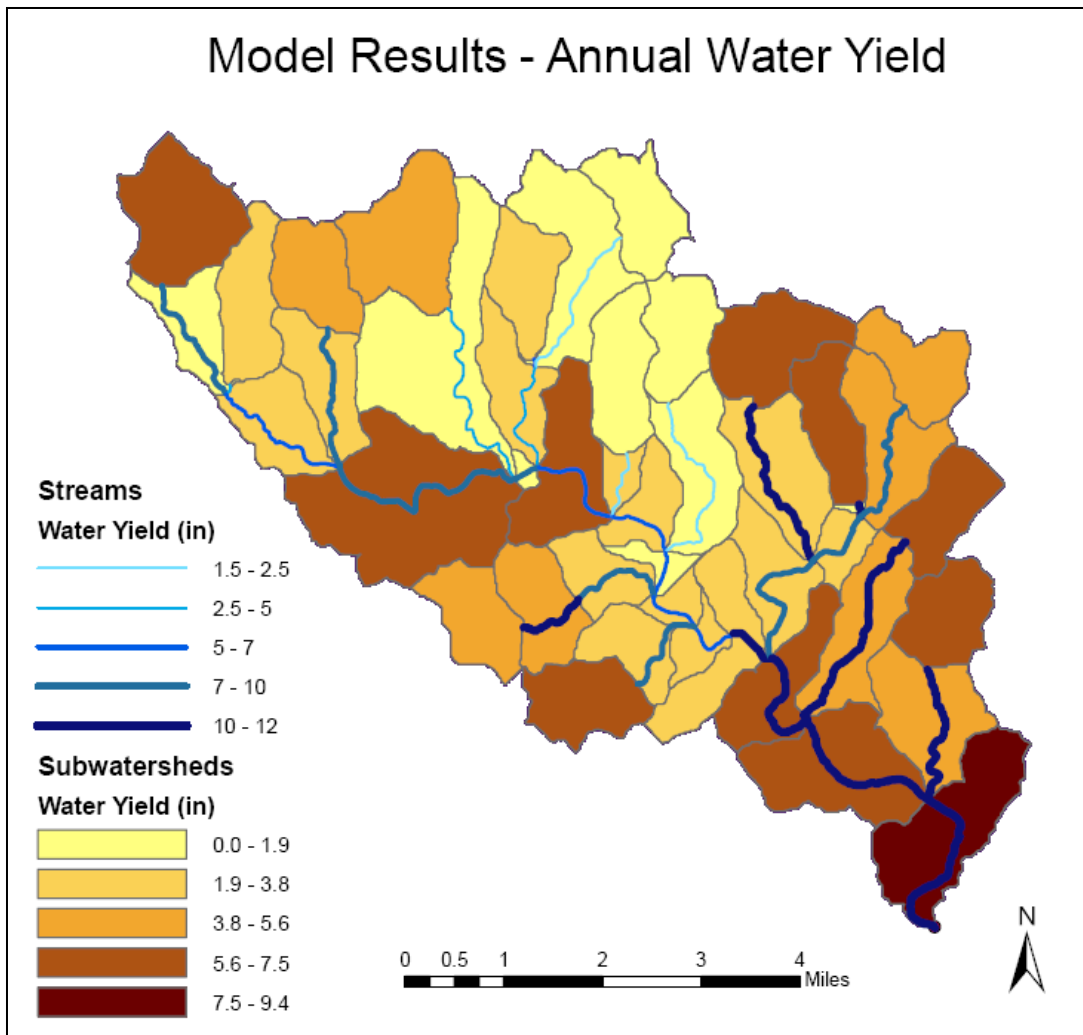
Figure 4.9. Simulated average water yield by subwatershed and reach, 2000-2009, using the SWAT hydrologic model.
