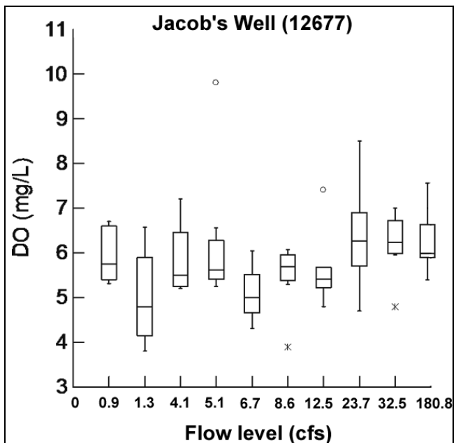
Figure 6.14. DO concentrations at Jacob's Well by flow level.
