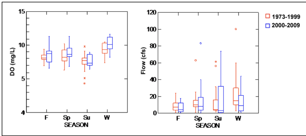
Figure 6.19. Box-and-whisker plots of DO and instantaneous flow (1973-1999 and 2000-2009)
