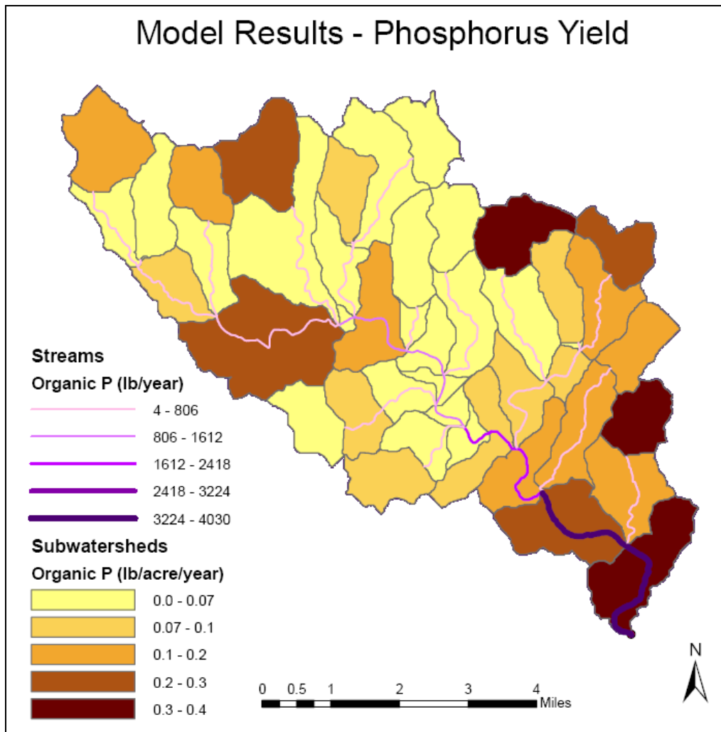
Figure 4.12. Simulated average organic phosphorus yield by subwatershed and reach, 2000-2009, using the SWAT hydrologic model.
