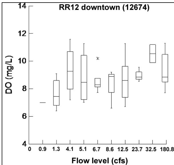
Figure 6.17. DO concentrations at the downtown Wimberley site by flow level.
